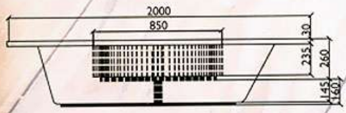
FRONT ELEVATION
