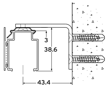
wall mounting with 2015-05
