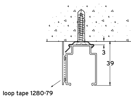
ceiling mounting with 7950
