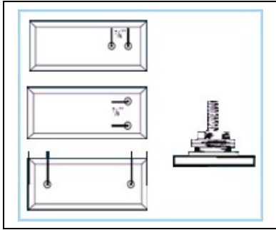
Post Terminal Dimension and Location
