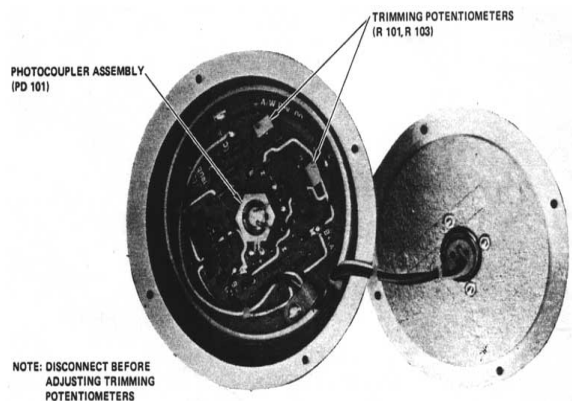
Scanner Housing Electronics
