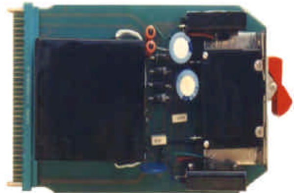
Power Supply card for Safe Flame II
