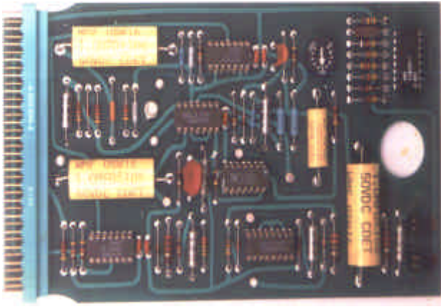
2/4 Flame Indication & Fault Alarm Card
