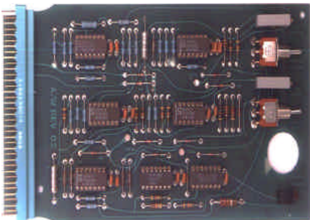
Intensity & Fault Alarm Card for Safe Flame II
